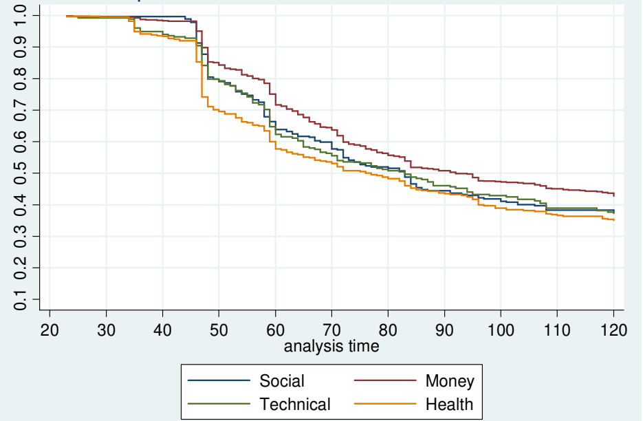
Kaplan-Meier survival estimates, TurkMoroc
