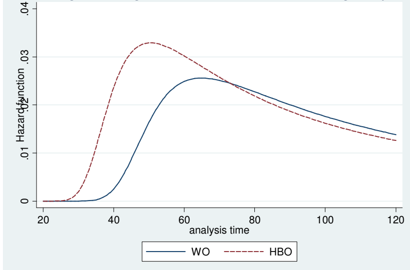
Generalized gamma regression with unobserved heterogeneity, MEN
