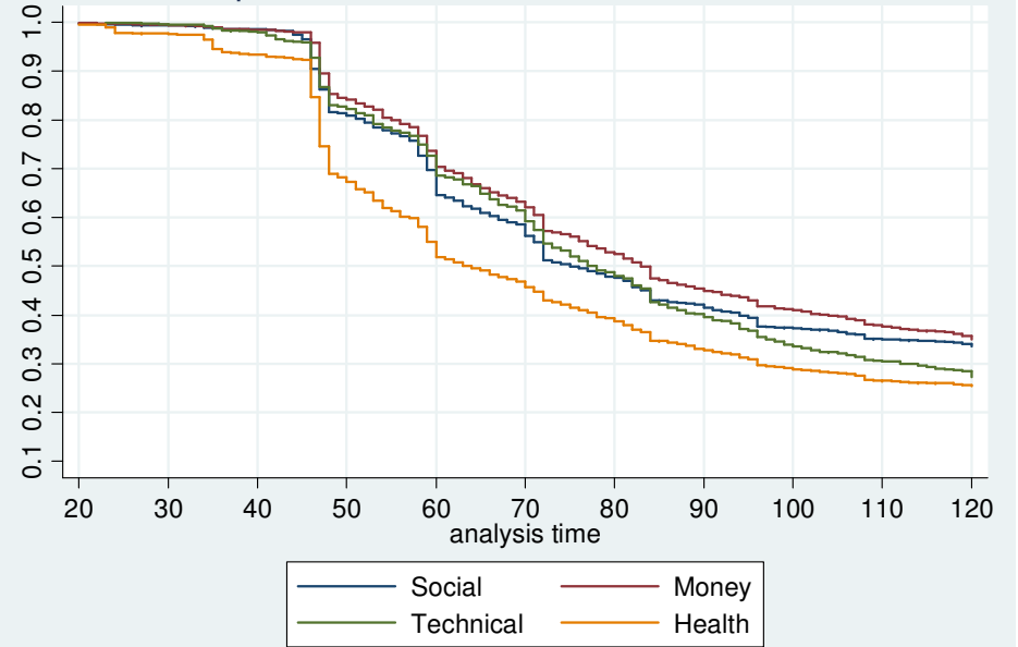
Kaplan-Meier survival estimates, Western
