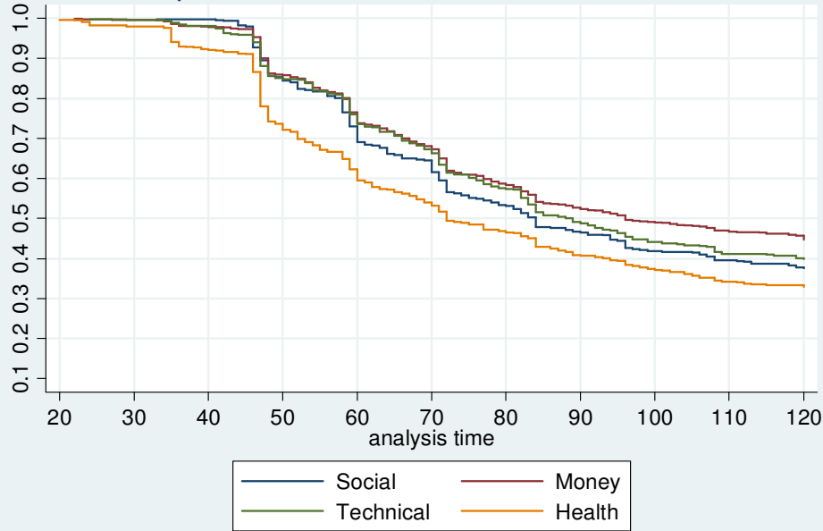
Kaplan-Meier survival estimates, Caribbean
