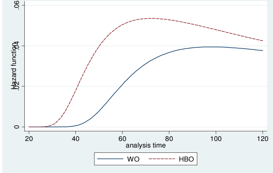
Generalized gamma regression with unobserved heterogeneity, MEN
