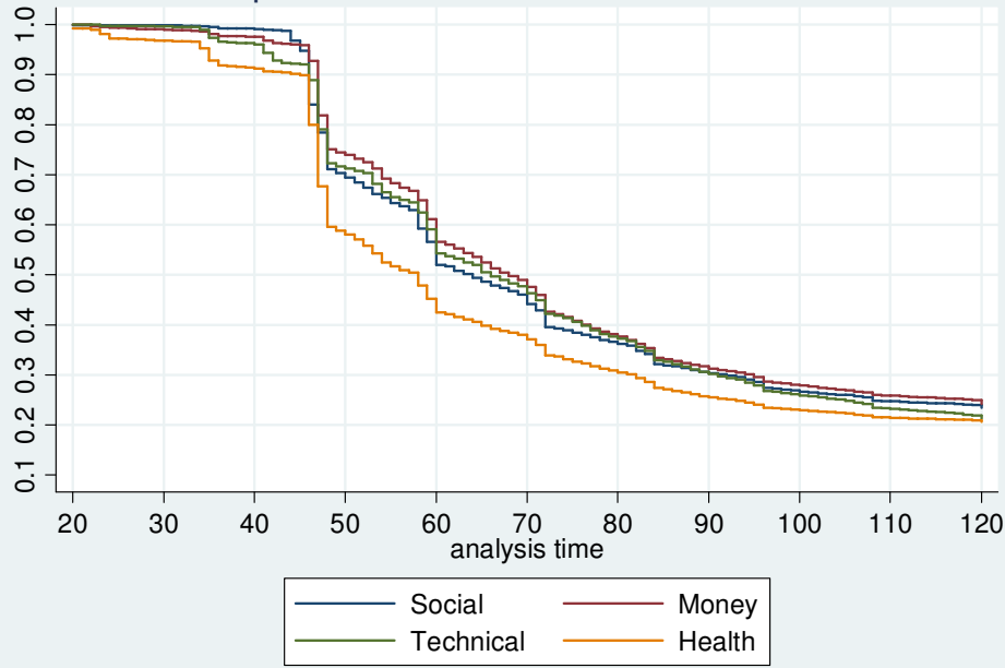
Kaplan-Meier survival estimates, Dutch
